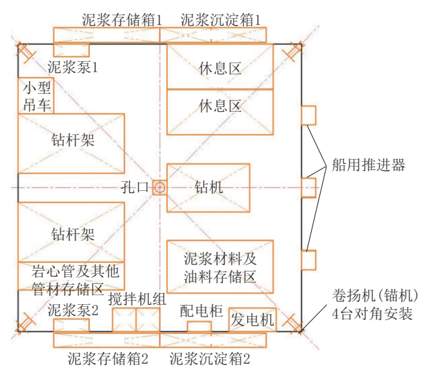
图 2 水上钻探平台布置 Fig.2 Layout of waterborne working platform
