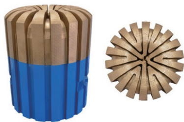
图7 \text{O}406\text{ mm} 表孕镶金刚石全面钻进钻头 Fig.7 \text{O}406\text{ mm} diamond full face drilling bit
