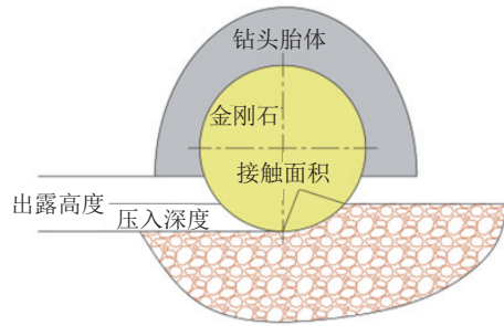
图5 金刚石钻头工作过程示意 Fig.5 Working process of the diamond bit
